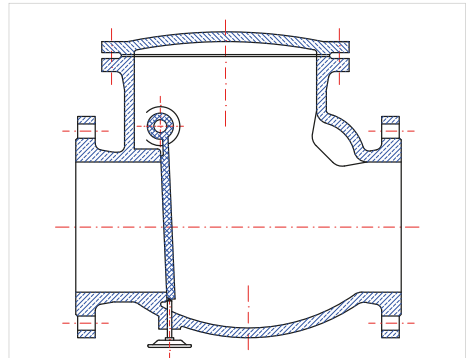
■ RFS mit Anlüftvorrichtung / RFS with mounted lifting device
